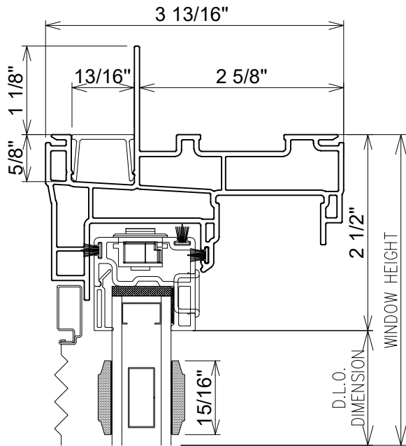
1 HEAD SECTION
