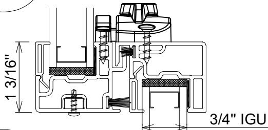
2 MEETING RAIL SECTION
