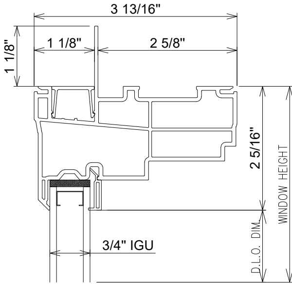
1A/1SP PW/CT HEAD SECTION
