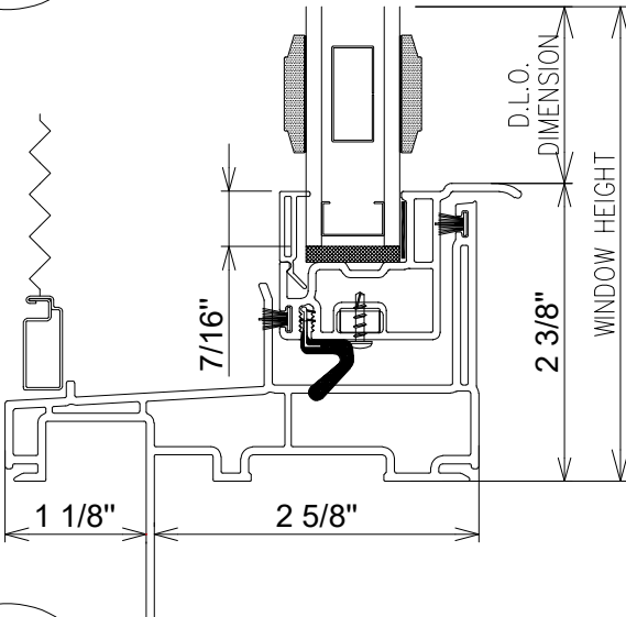
3 SILL SECTION
