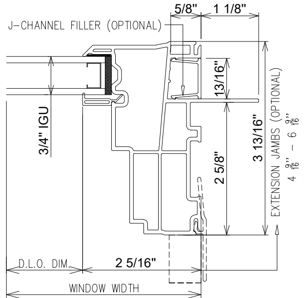
4A/6SP PW/CT JAMB SECTION
