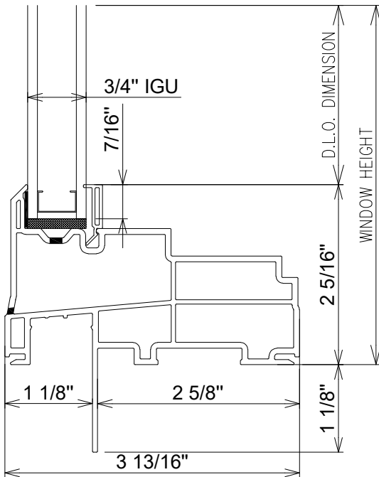
3A PW SILL SECTION
