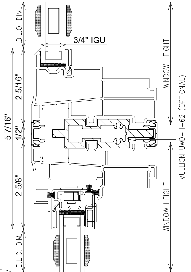
6A MULLION HORIZONTAL SECTION
